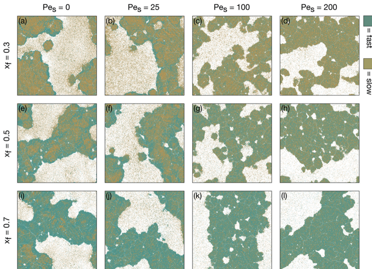
Fig. 3 Simulations of active Brownian particles with distinct slow (gold) and fast ( Pe_f = 500 , teal) particle fractions and activities. All snapshots were taken after steady-state had been reached, \tau_r = 300 . The particle fraction is constant in each row: x_f = 0.3 , 0.5, and 0.7; illustrating majority slow, equal and majority fast mixtures respectively. The activity of the slow species is constant in each column: Pe_s = 0 , 25, 100, and 200. The activity of the fast species is fixed at Pe_f = 500 .
