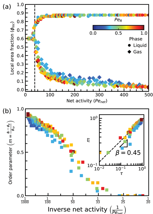
Fig. 6 Steady-state local area fraction of liquid (circles) and gas (diamonds) states outline a binodal when plotted against net activity (a). Dense phase approaches and does not exceed the close-packing area fraction of disks in two dimensions. Activity ratio (color), appears to account for minor deviations from complete collapse of the data. Vertical dashed line represents the critical activity as reported in ref. 47. Order parameter of systems at steady-state (b) where increasing the inverse net activity corresponds to a transition to the gas phase. (Inset) Determination of the critical exponent \beta with respect to the reduced inverse net activity ( m = (-\tau)^\beta ) gives \beta = 0.45 with residual r^2 = 0.93 for linear scales.
