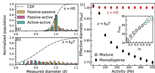
Fig. 1 Comparison of particle activity and interparticle distance for particle pairs within the WCA interaction cutoff ( 0 \leq r \leq r_{\text{cut}} ). (left) Histograms of the measured diameters as they occur in our simulations, separating interactions between passive-passive, passive-active and active-active, as well as showing the cumulative distribution function (CDF) overlaid. CDF displays the probability of a particle having diameter \leq x . Data are computed for an active/passive simulation with x_f = 0.1 and Pe_f = 500 . (a) Histogram and CDF for simulations performed using \varepsilon from eqn (6) demonstrates that no particles have measured diameter \delta \leq 0.95 while 50% of particles have measured diameters 0.95 < \delta \leq 1.00 . (b) Histogram and CDF for simulations using \varepsilon = k_B T where all types of interaction data deviate well below the intended diameter. (c) Plot of the effective diameter measured in simulation as a function of particle activity. Simulation data for monodisperse simulations with well depth \varepsilon = k_B T (black) shows drastic particle overlap as activity is increased. Data for systems simulated with interaction potential according to eqn (6) (red), maintains a constant mode center-to-center distance that is equal to the intended diameter ( = 1 for hard spheres). Inset shows predicted \varepsilon both from eqn (6) (dashed line) and computed from emergent simulation data with respect to system composition. Required well depth is computed for passive-passive (gold), passive-active (pink), and active-active (teal) interactions.
