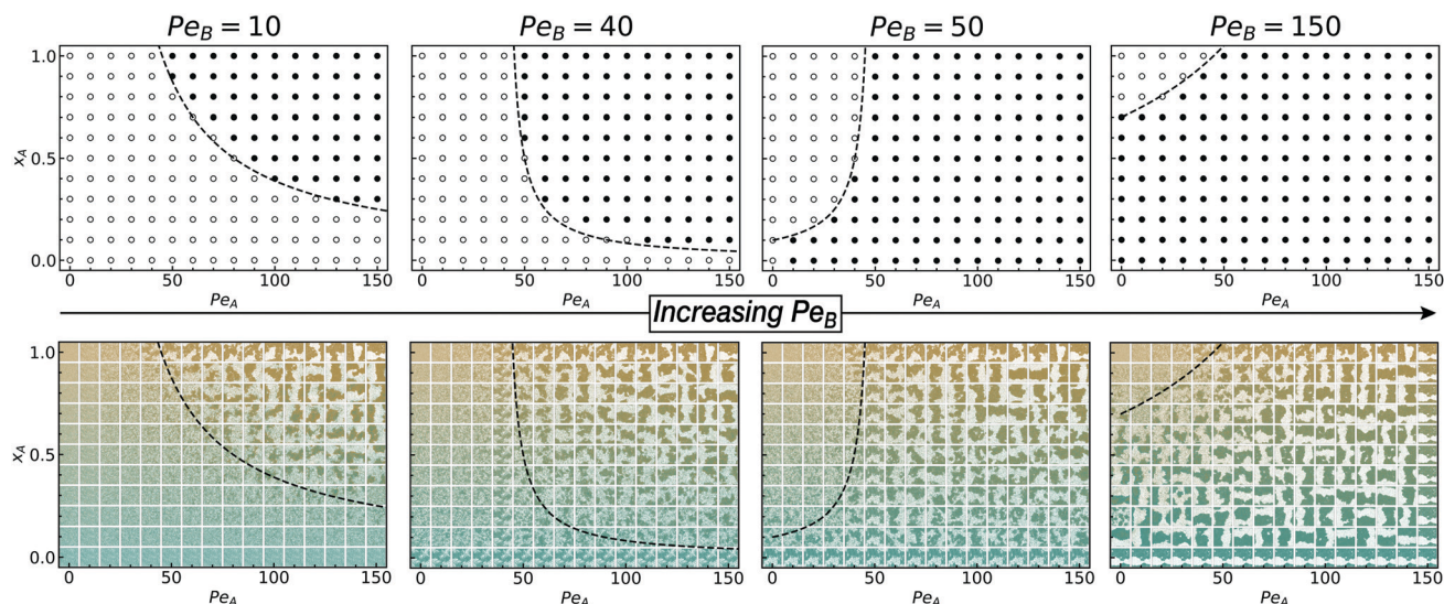
Fig. 2 Top row: Phase diagram in the x_A – Pe_A plane for Pe_B = 10, 40, 50, 150 . Filled symbols denote phase-separated systems, as determined by our MIPS-identifying algorithm, and open symbols denote a gaseous steady-state. The dashed lines indicate phase boundaries predicted by the active/active equation for \phi_0 in Table 1, which is the theoretical binodal according to our kinetic theory. There is good agreement between the simulations and theory. Bottom row: The same phase diagrams are shown illustrated by simulation (final) snapshots after 300\tau_r , where ‘A’ particles are shown in gold and ‘B’ particles in teal. (See ESI, † Fig. S2 for the full parameter range.)
