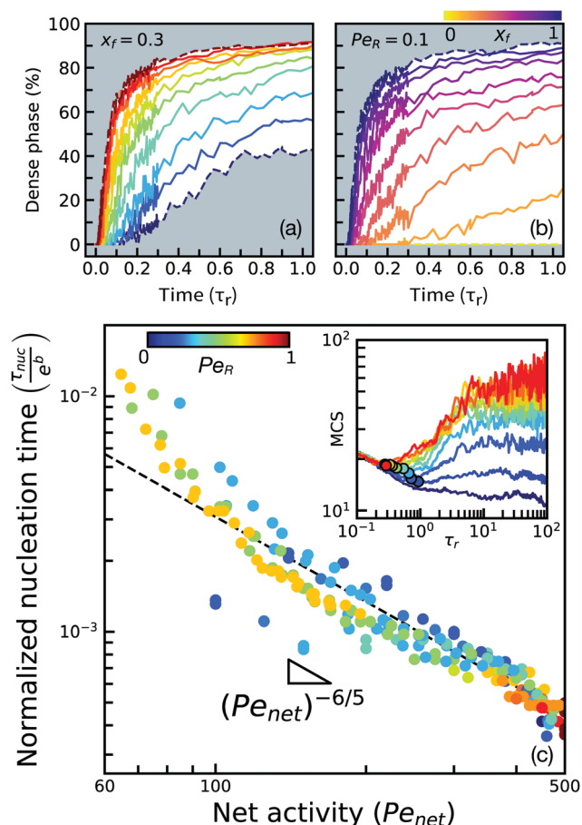
Fig. 5 Time-resolved participation of all particles in the dense phase at constant particle fraction ( x_f = 0.3 ) showing the effect of changing slow particle activity is shown in (a). Colorbar indicates the activity ratio of each simulation ( Pe_f = 500 ). Constant activity ratio (b, Pe_R = 0.1 ) illustrates the effect of varying the particle fraction (where shade indicates each simulated particle fraction and dashed lines indicate monodisperse systems). Dynamic data shows a power-law relationship between nucleation time and net activity (c). Nucleation time is normalized by a constant ( e^b ) for each value of the activity ratio to emphasize the common slope of the data. Points are collapsed from a wide variety of activity ratios ( Pe_R ), particle fractions ( x_f ), and fast particle activities ( Pe_f ). Inset shows computation of the nucleation time, taken as the local minimum in the mean cluster size vs. time.
