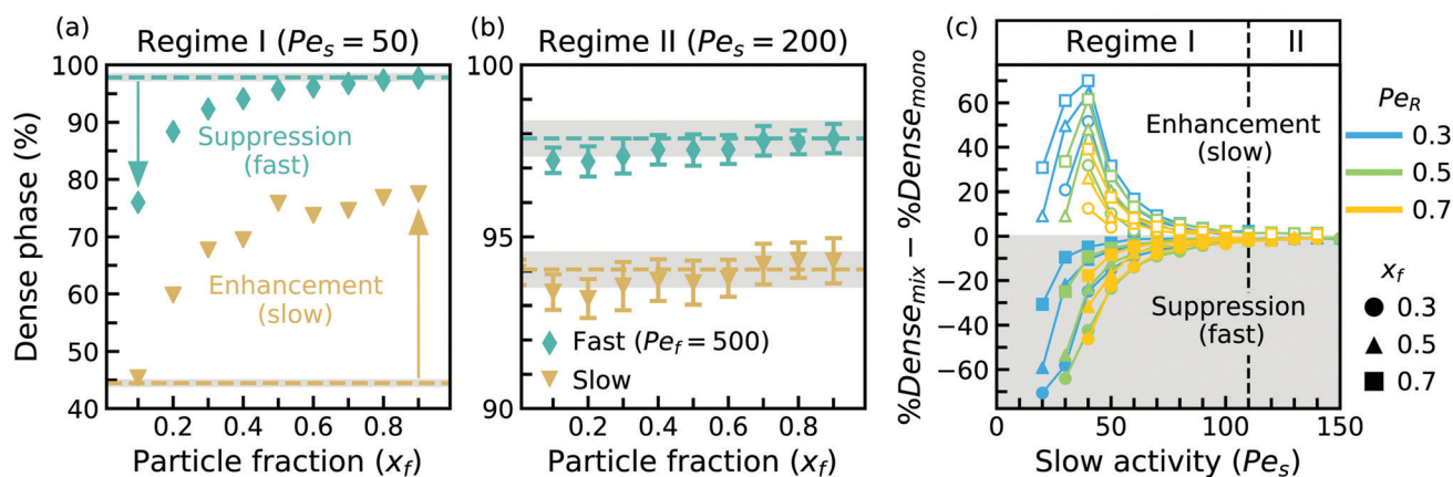
Fig. 4 Steady-state participation in the dense phase for both fast and slow species. (a and b) Percentage of each particle type in the dense phase for different particle fraction in (a) regime I ( Pe_s = 50 ) and (b) regime II ( Pe_s = 200 ) compared to a monodisperse system of each particle type (dashed lines). Error bars are shown when larger than the symbol size and in grey shading for monodisperse systems. (a) In regime I slow species experience enhancement and fast species exhibit suppression with respect to a monodisperse system of the same total area fraction. (b) In regime II fast and slow species assume the dense phase participation (within error) of a monodisperse fast or slow system respectively. These data are condensed in (c) a plot of the difference in the percent participation in the dense phase between a mixed and monodisperse system at distinct activity ratios and particle fractions. Negative values (filled symbols) indicate suppression of the fast component and positive values (unfilled symbols) show enhancement of the slow component. Regime I persists for systems that undergo MIPS with slow activity up to Pe_s \approx 110 and activity ratio less than unity. Beyond this point, each species assumes the steady-state participation in the dense phase correspondent to a monodisperse simulation at the same activity and total system area fraction.
