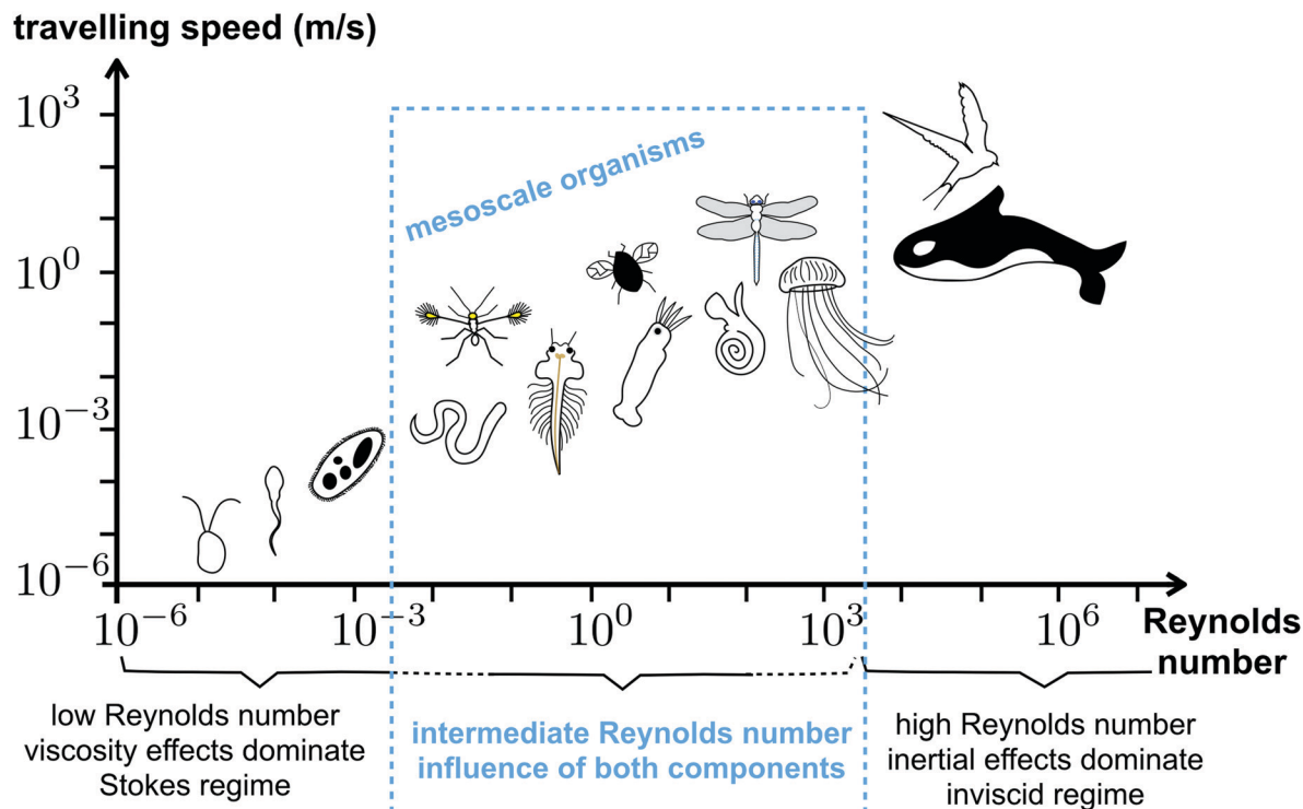
Fig. 1 Reynolds numbers in the animal kingdom, highlighting the intermediate Reynolds range for swimming and flying organisms. The organisms shown schematically from low to high Reynolds numbers are: algae, bacterium, paramecium, nematode, fairyfly, brine shrimp, larval squid, wasp, pteropod, dragonfly, jelly fish, whale, swallow. Layout inspired by Nachtigall. 8
